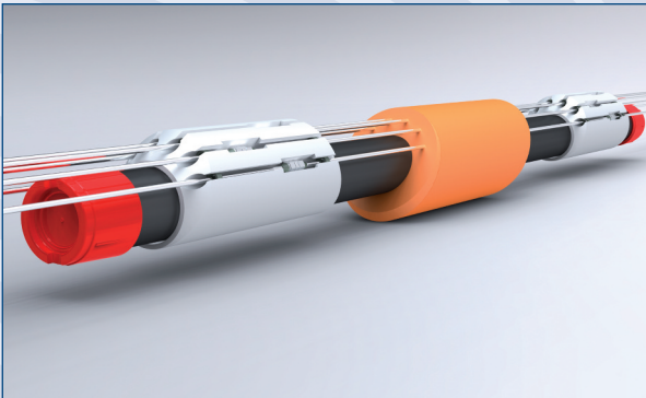
SIS multi element design with an example of cable feed through
